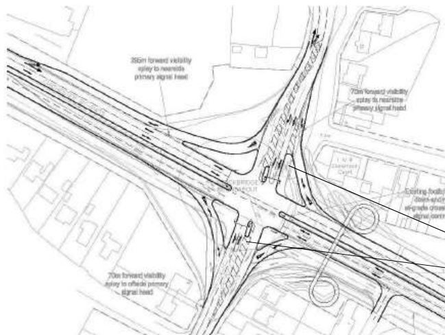
Figure 7.5: Stockbridge Junction Proposed Mitigation
